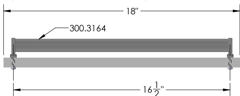
Mounting Hole Position on Shelf
