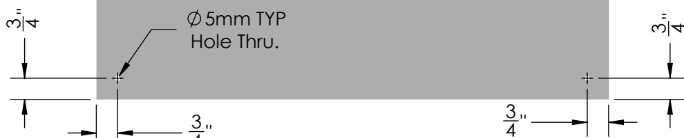
Mounting Hole Position on Shelf
